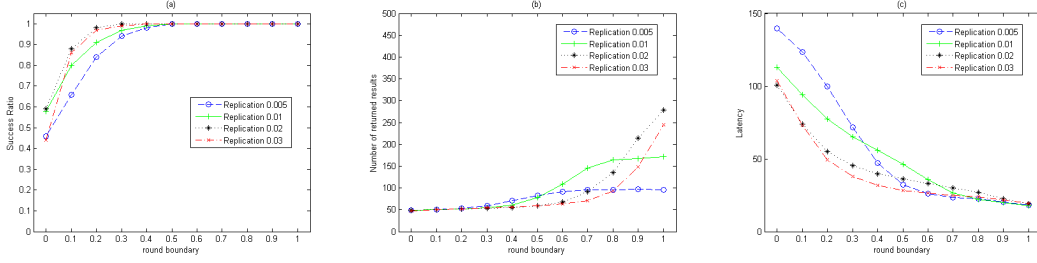
Fig. 4. Rounding Boundary impact to DQ(i)+: Confidential Parameter 2
