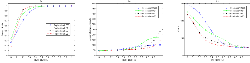
Fig. 5. Rounding Boundary impact to DQ(i)+: Confidential Parameter 3
