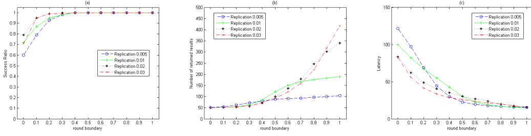
Fig. 3. Rounding Boundary impact to DQ(i)+: Confidential Parameter 1
