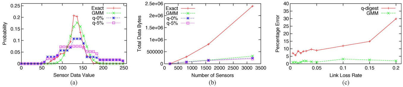
Fig. 1. Performance comparison of the algorithms in the presence of link failures. (a) Histograms (5% link failures). (b) Communication cost (5% link failures). (c) Error rates.
