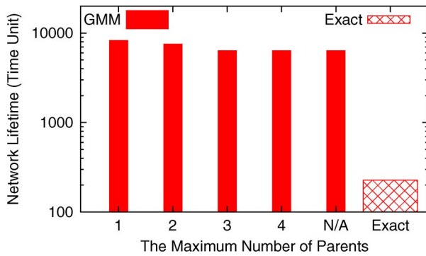
Fig. 8. Network lifetime comparison.
