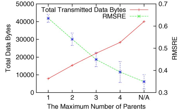
Fig. 7. Tradeoff between the accuracy and the message cost.
