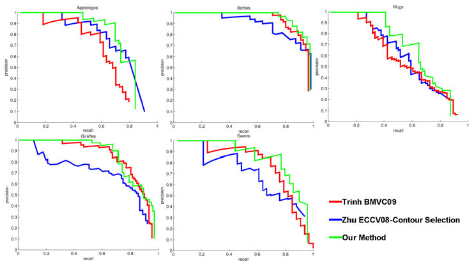
Fig. 10. Precision/Recall curves of our method fig compared to [28] and [26] for 5 classes of ETHZ dataset
